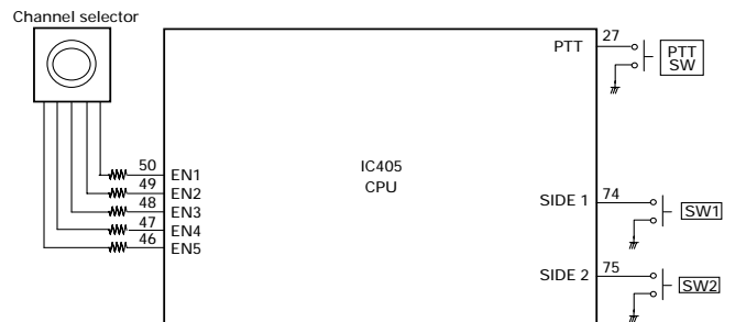
Fig. 11 Control system
